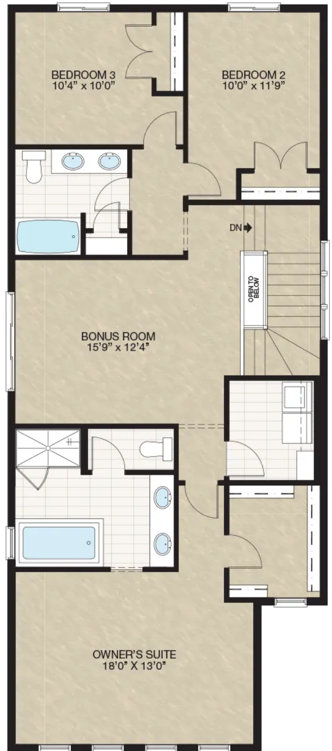
UPPER 1280 SQ.FT.
