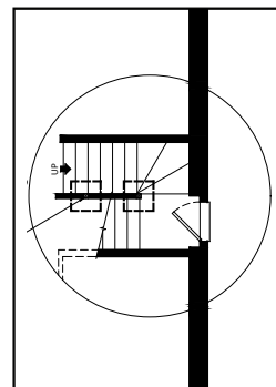
SIDE ENTRY WITH REVISED BASEMENT STAIRS
