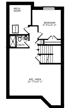
1 BEDROOM 'LEGAL SUITE' 704 SQ FT
